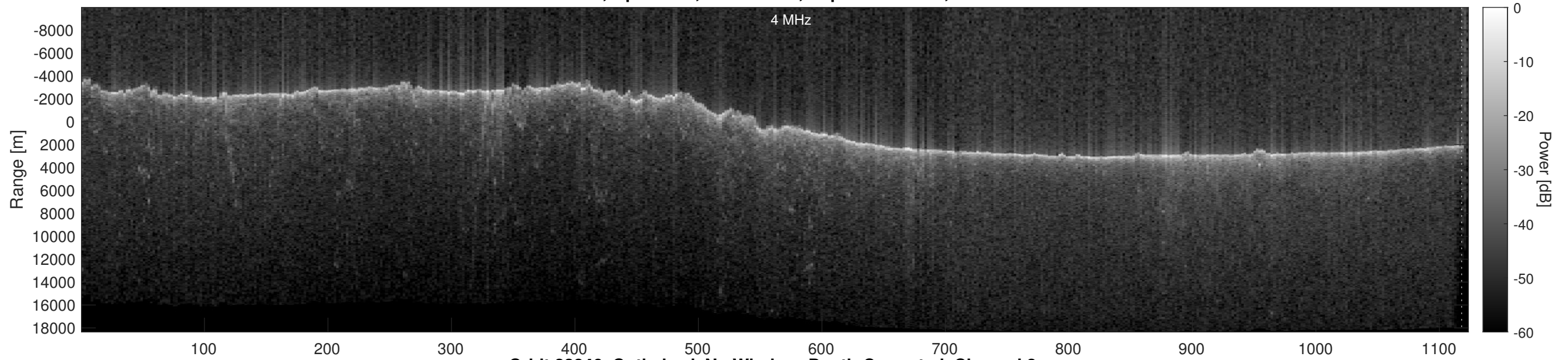
Orbit 22846, Optimized, No Window, Depth-Corrected, Channel 2
