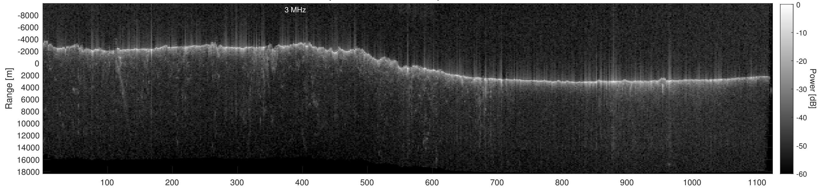
Orbit 22846, Depth-Corrected Cluttergram
