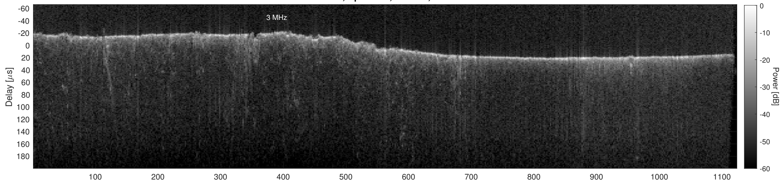
Orbit 22846, Cluttergram
