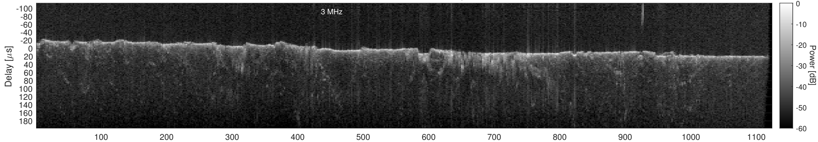
Orbit 22847, Cluttergram
