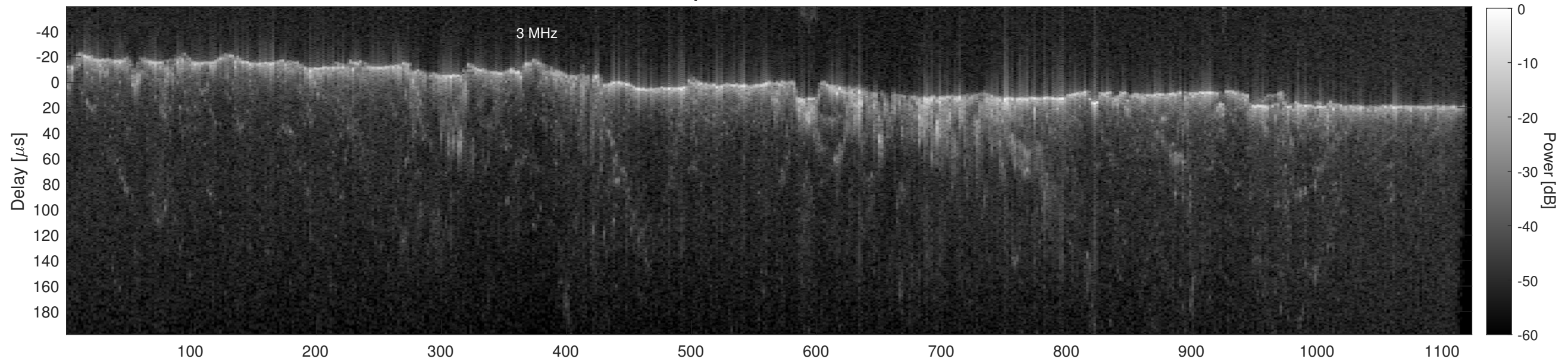
Orbit 22847, Cluttergram
