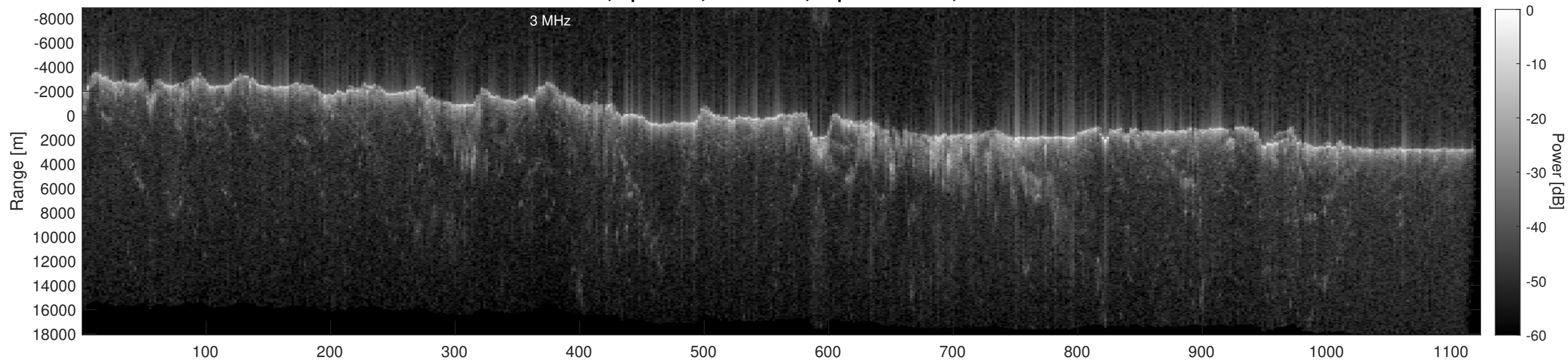
Orbit 22847, Depth-Corrected Cluttergram
