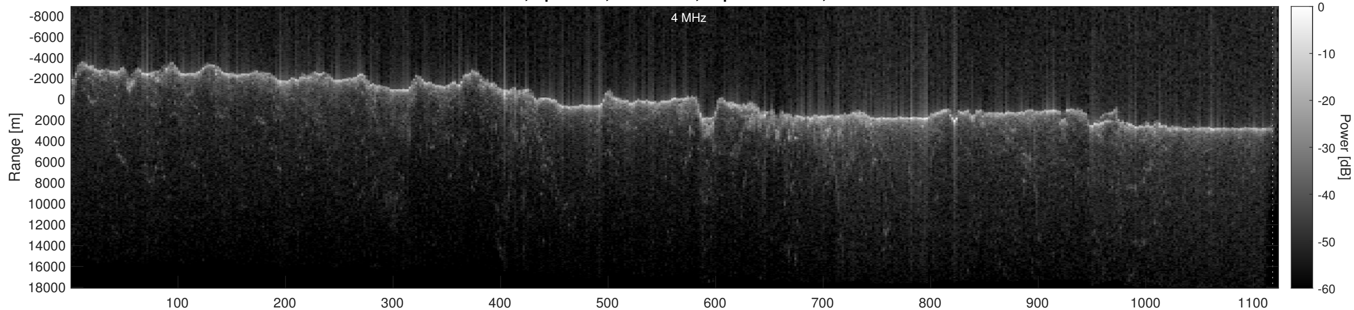
Orbit 22847, Optimized, No Window, Depth-Corrected, Channel 2
