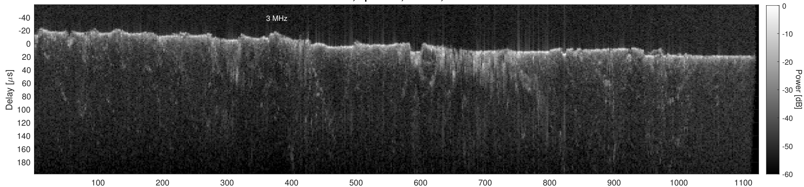
Orbit 22847, Cluttergram
