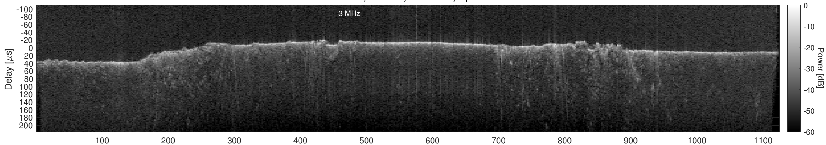
Orbit 22850, Cluttergram
