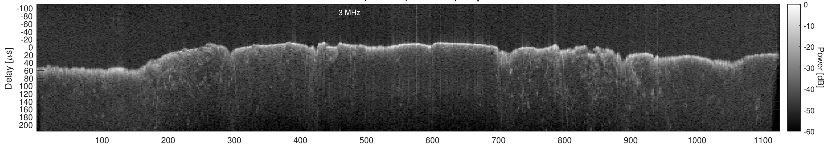
Orbit 22850, Window, Channel 2, Optimized
