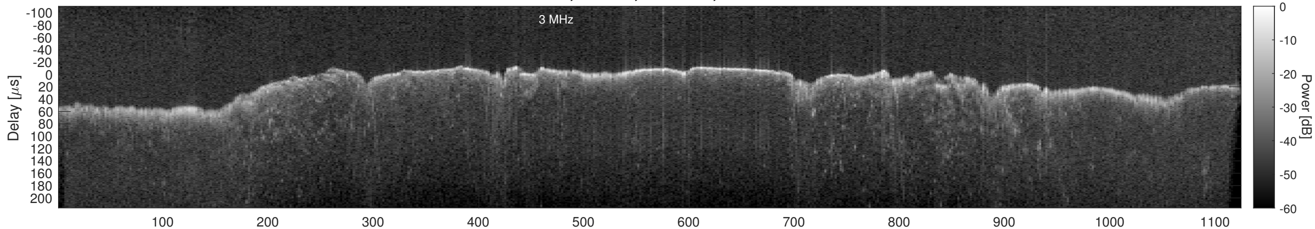
Orbit 22850, Window, Channel 2, Chapman
