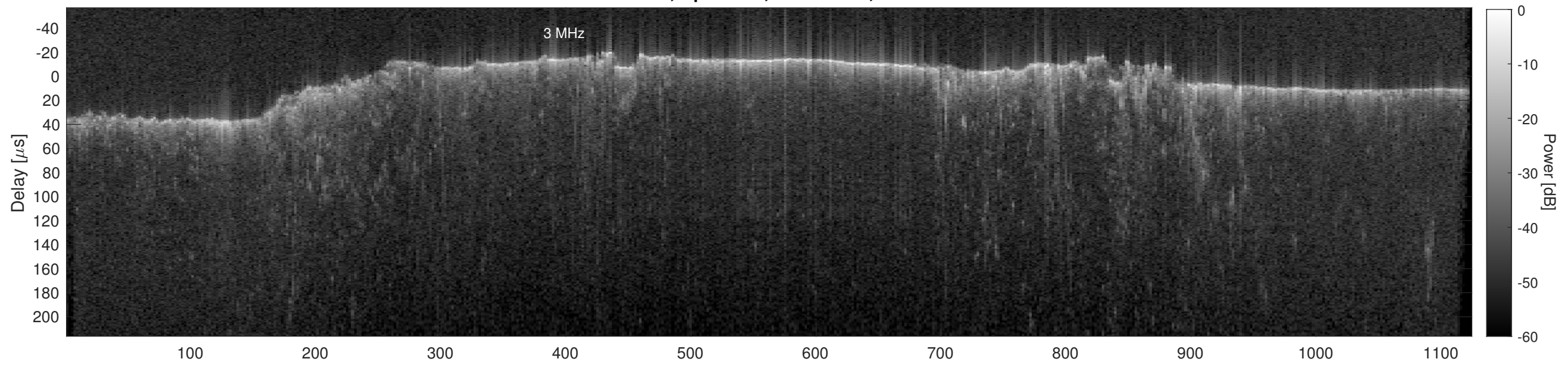
Orbit 22850, Cluttergram
