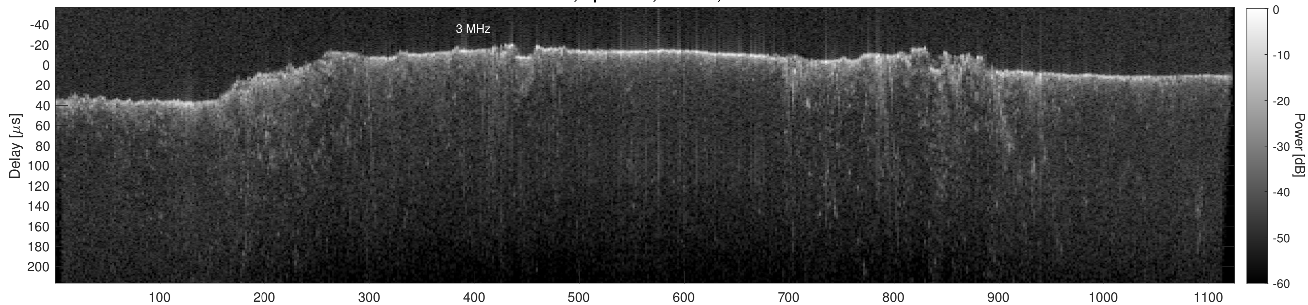
Orbit 22850, Cluttergram
