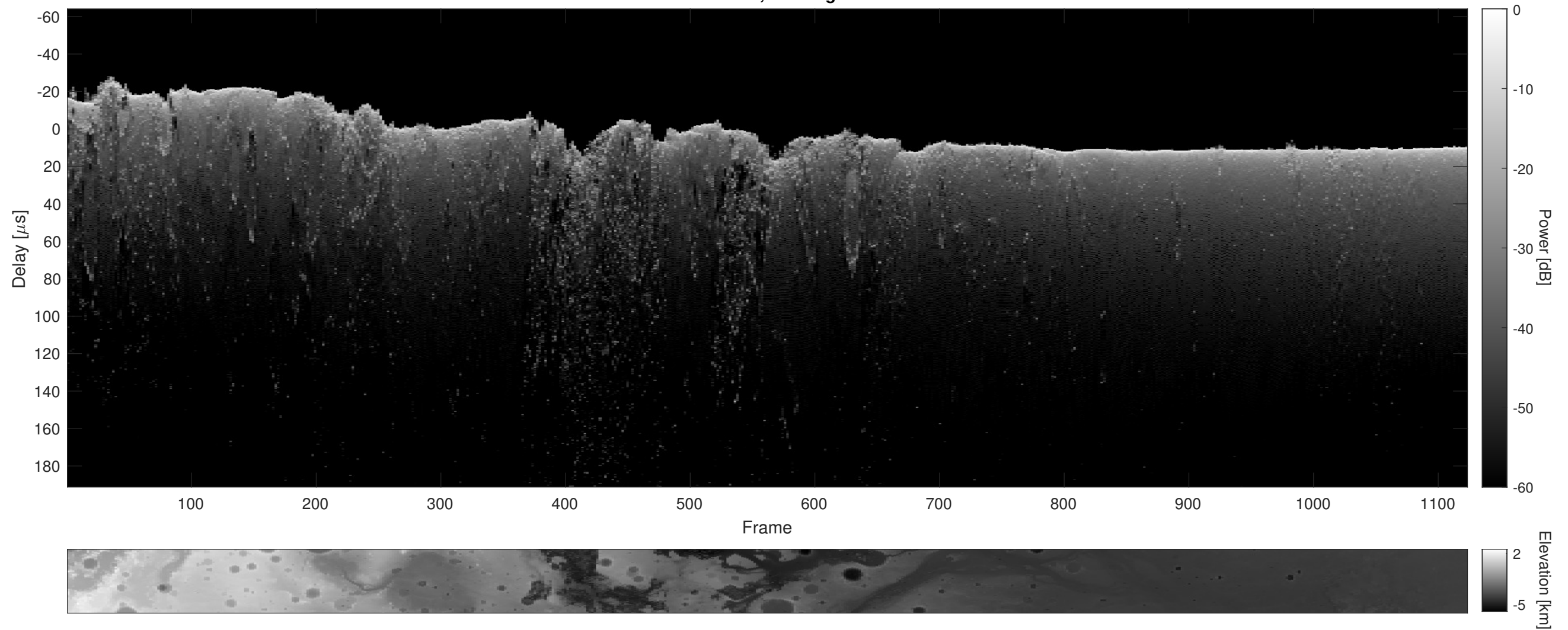
Orbit 22851, Cluttergram
