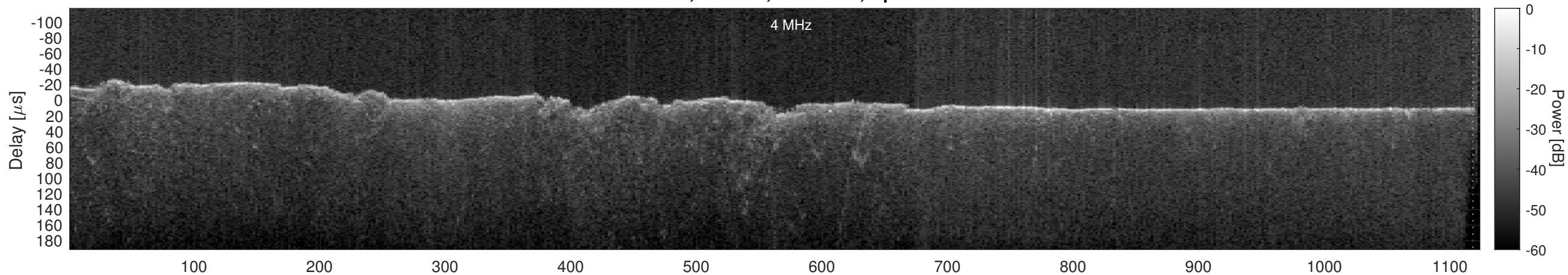
Orbit 22851, Cluttergram
