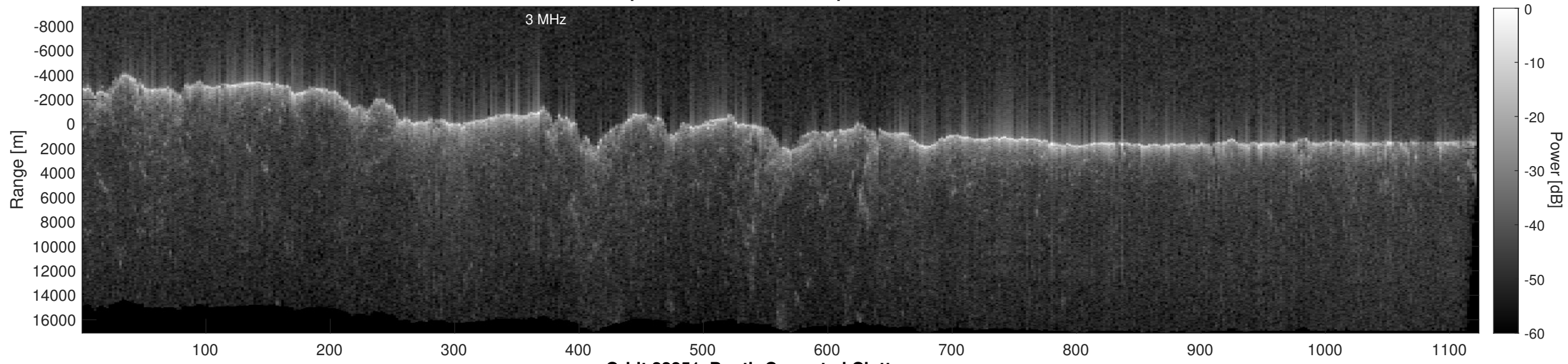
Orbit 22851, Depth-Corrected Cluttergram
