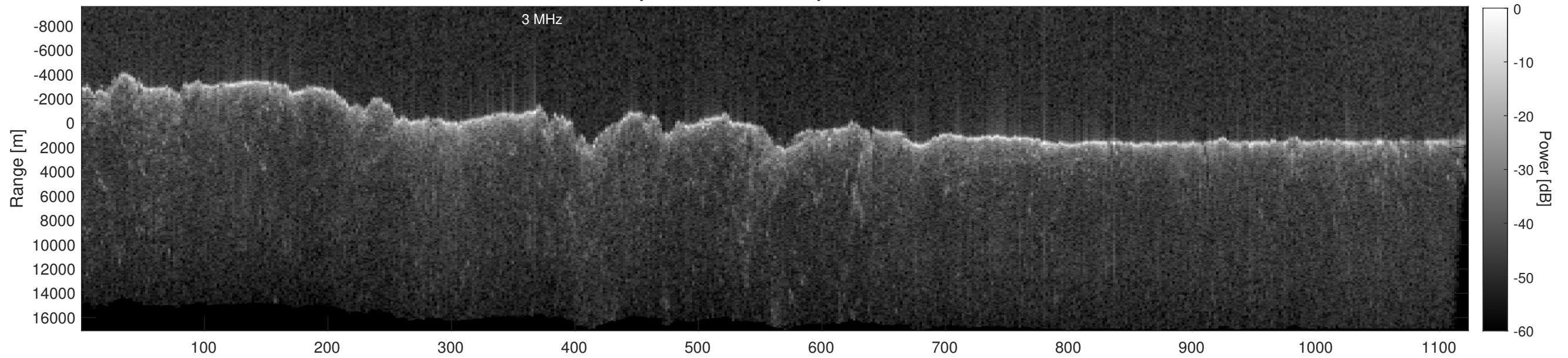
Orbit 22851, Depth-Corrected Cluttergram
