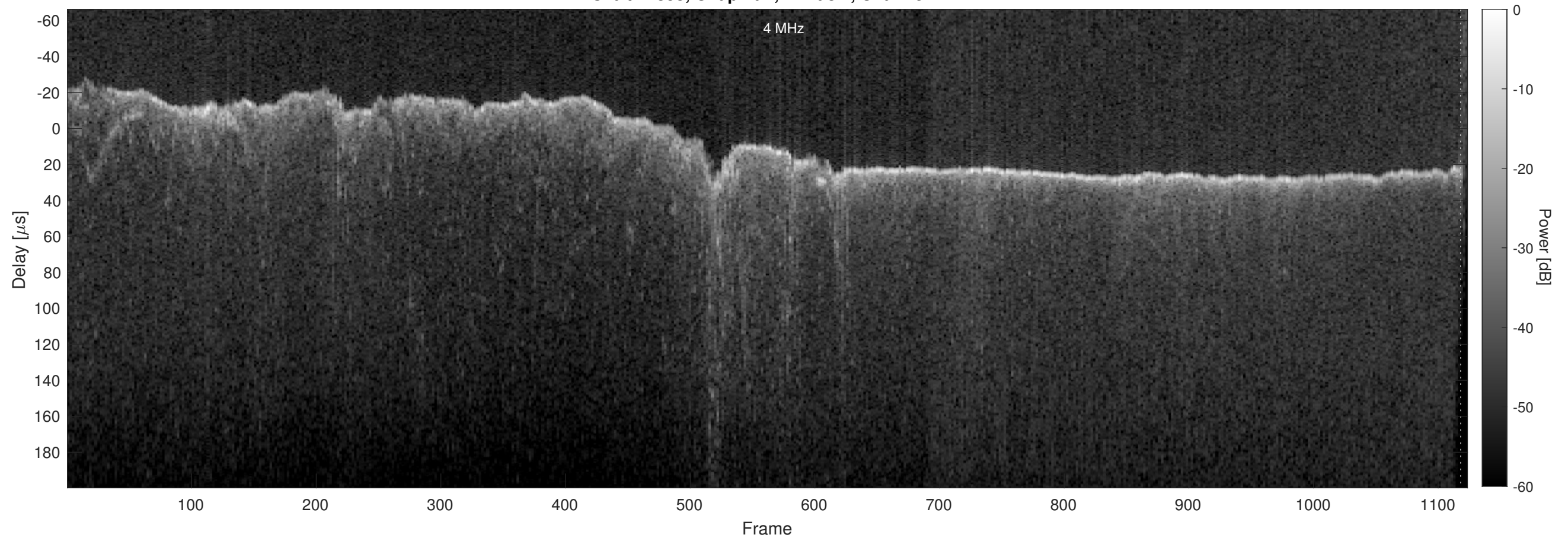
Orbit 22853, Chapman, Window, Channel 2
