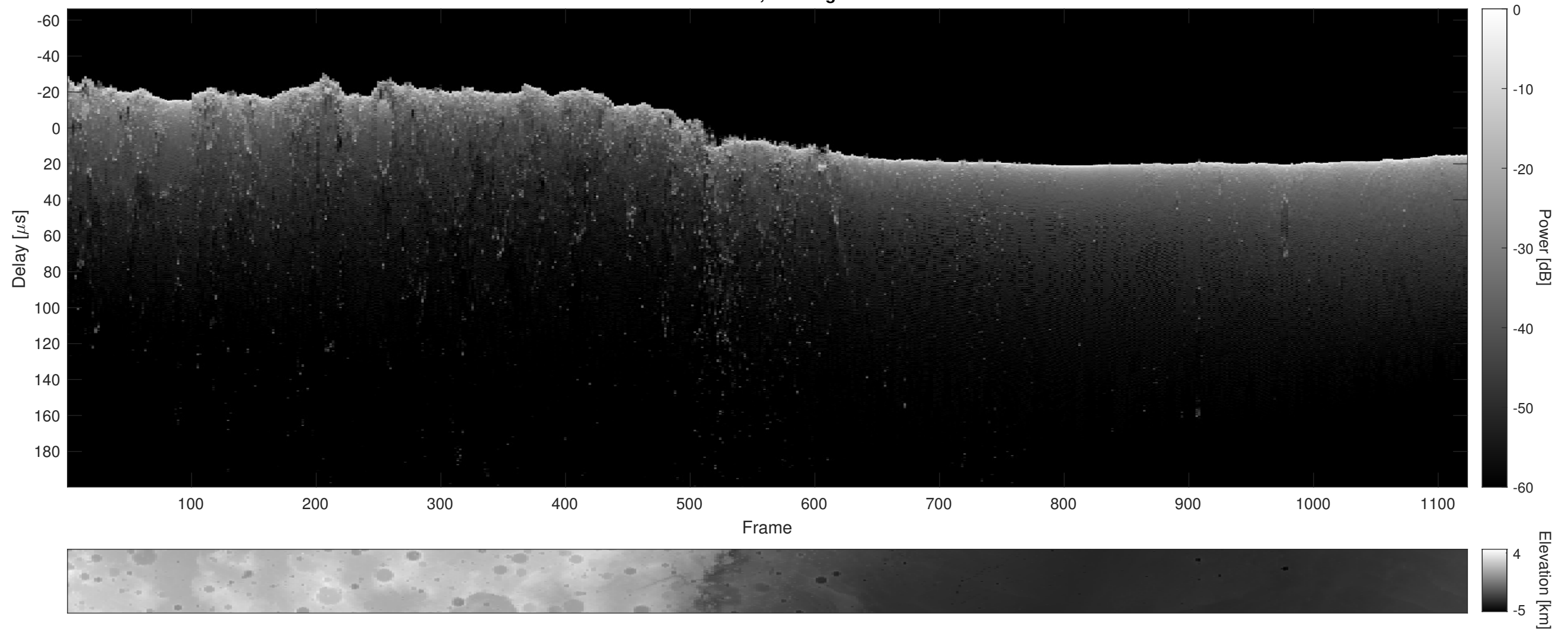
Orbit 22853, Cluttergram
