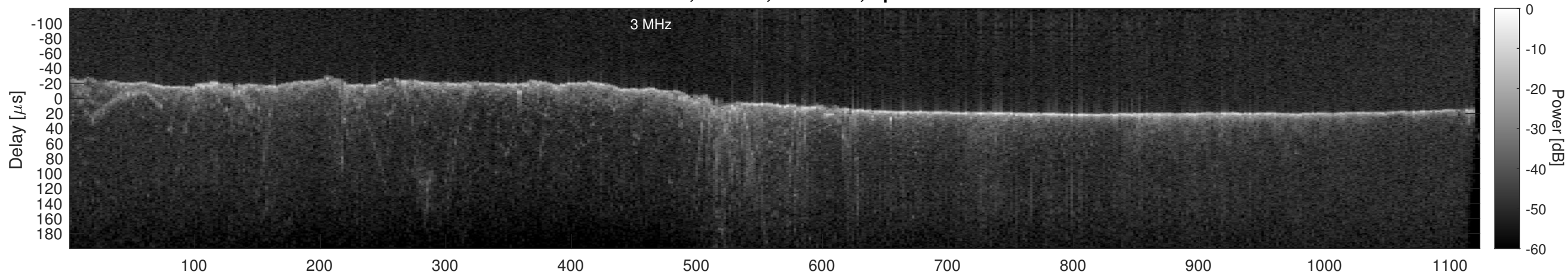
Orbit 22853, Cluttergram
