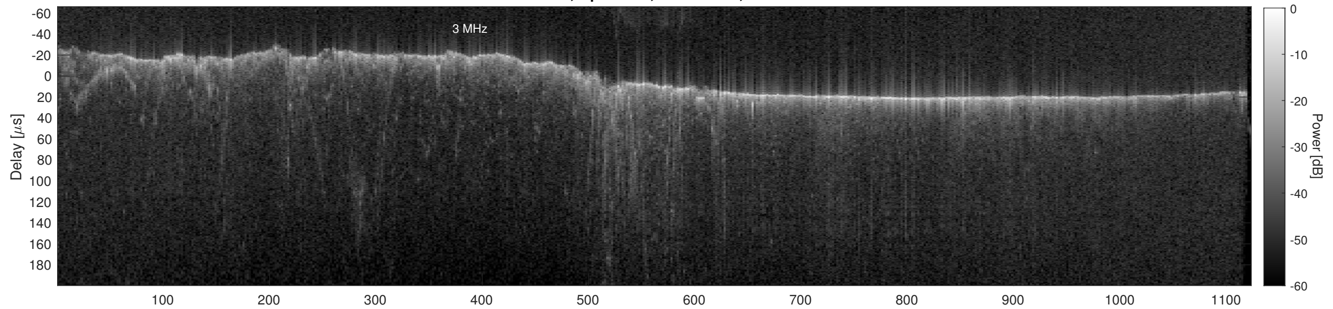
Orbit 22853, Cluttergram
