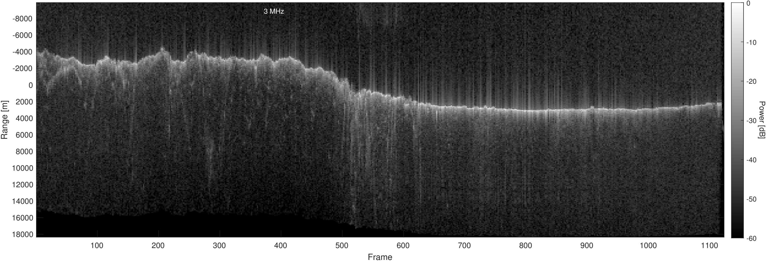
Orbit 22853, Optimized, No Window, Depth-Corrected, Channel 2
