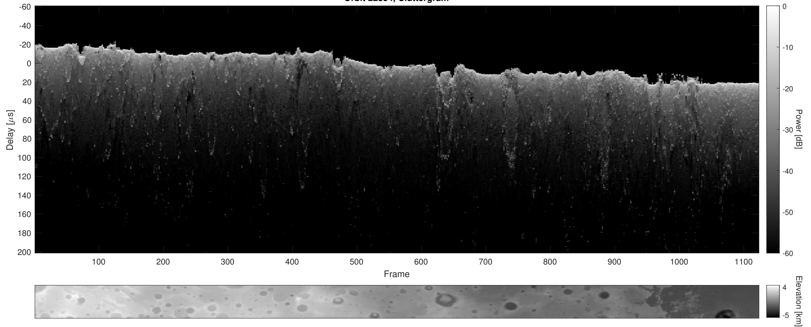
Orbit 22854, Cluttergram
