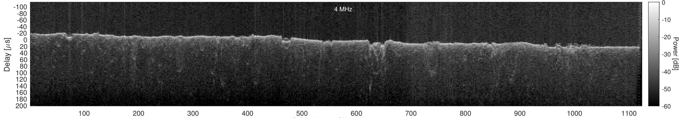
Orbit 22854, Cluttergram
