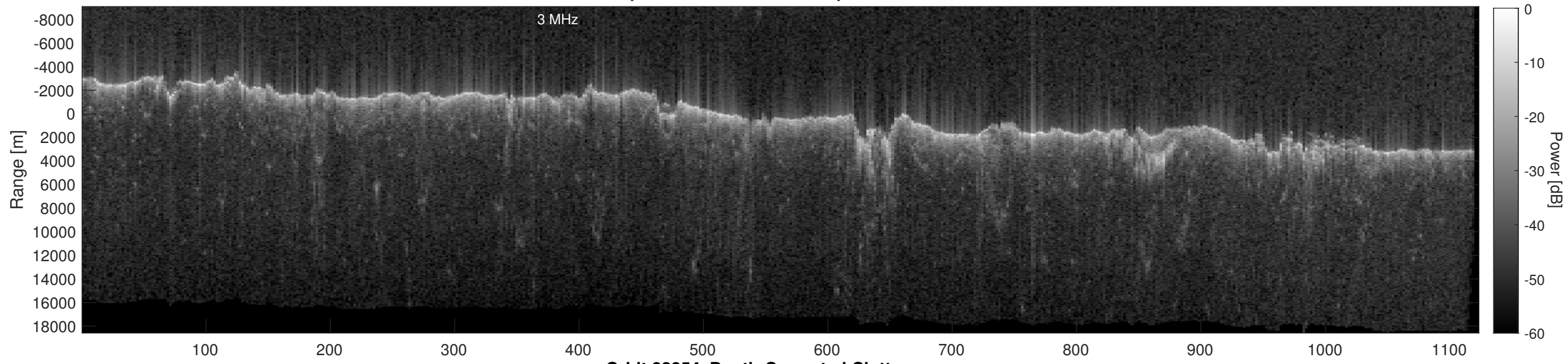
Orbit 22854, Depth-Corrected Cluttergram
