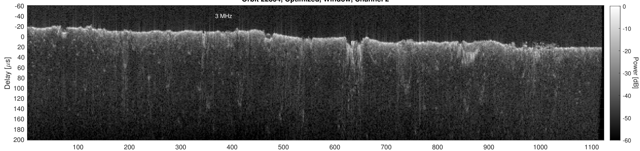
Orbit 22854, Cluttergram
