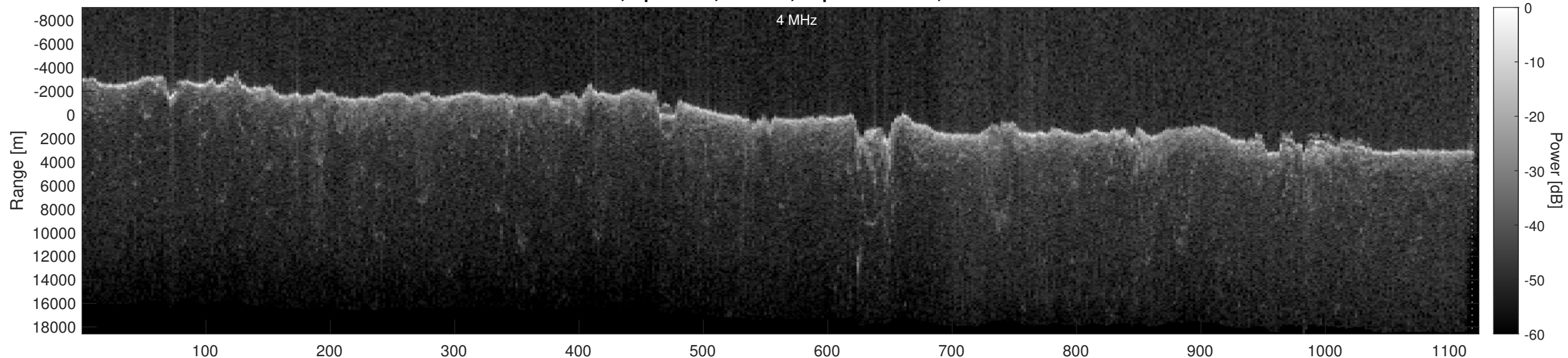
Orbit 22854, Optimized, Window, Depth-Corrected, Channel 2
