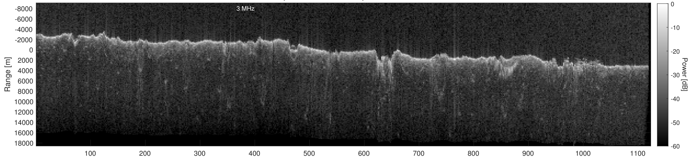
Orbit 22854, Depth-Corrected Cluttergram
