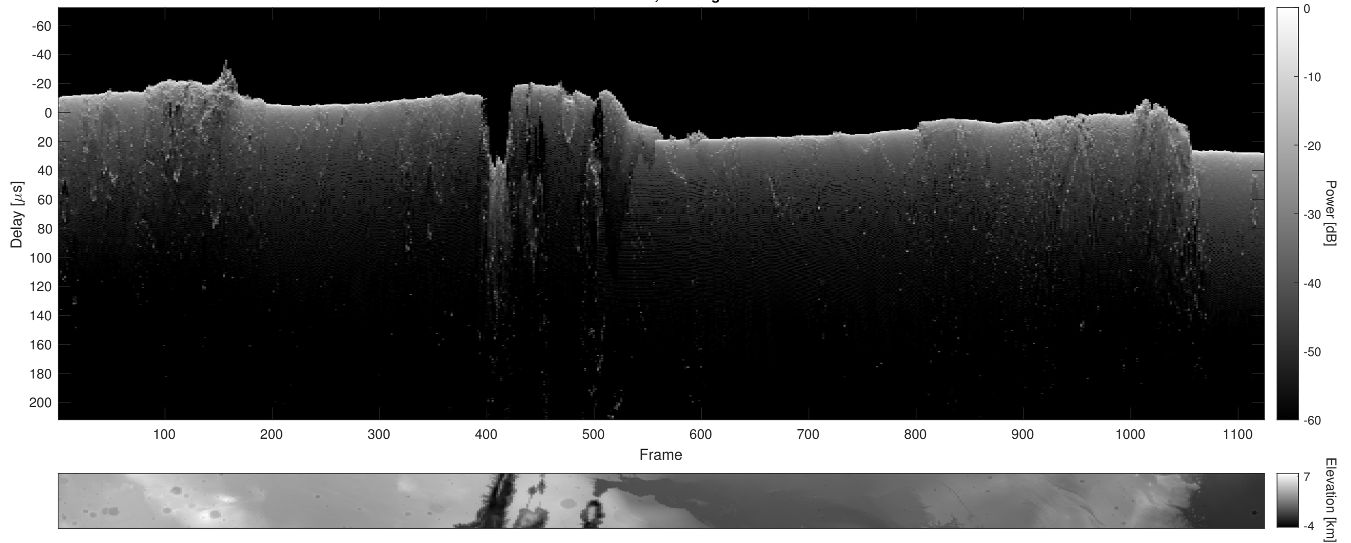
Orbit 22855, Cluttergram
