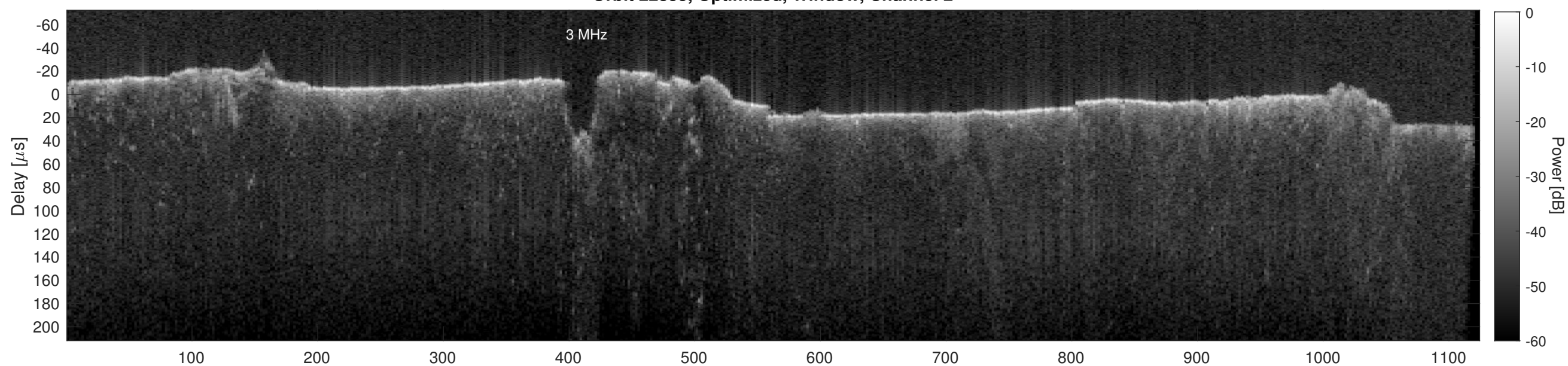
Orbit 22855, Cluttergram
