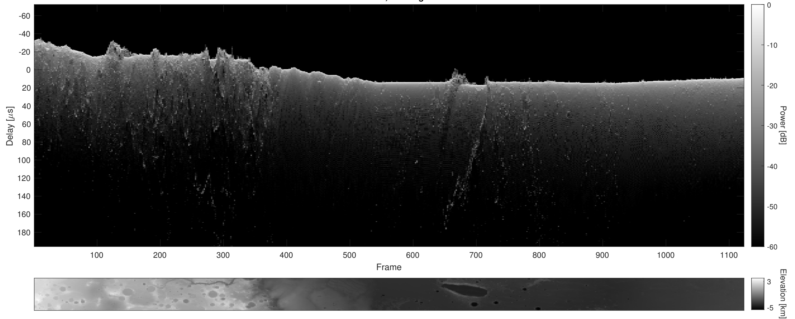
Orbit 22856, Cluttergram
