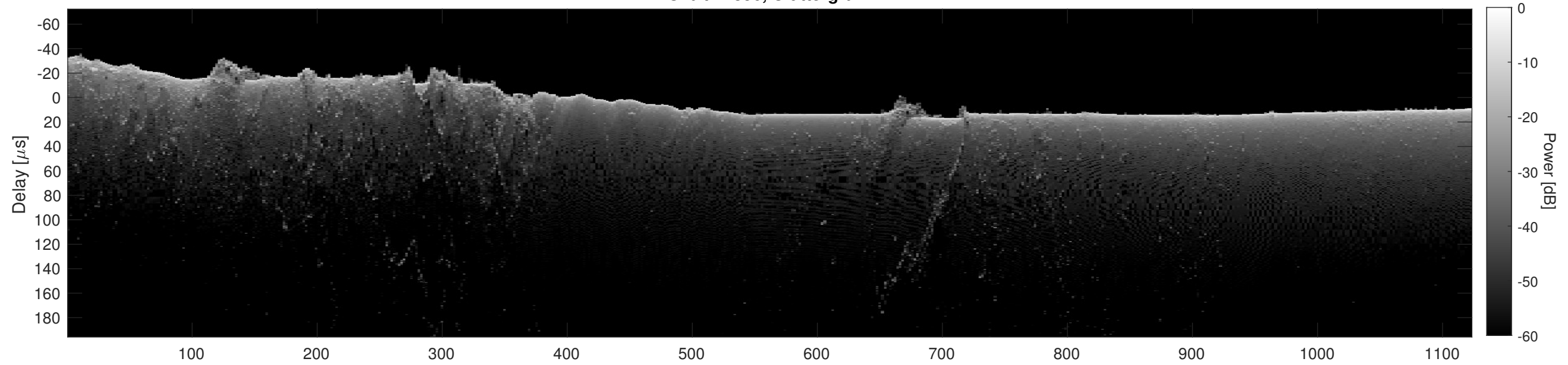
Orbit 22856, Cluttergram
