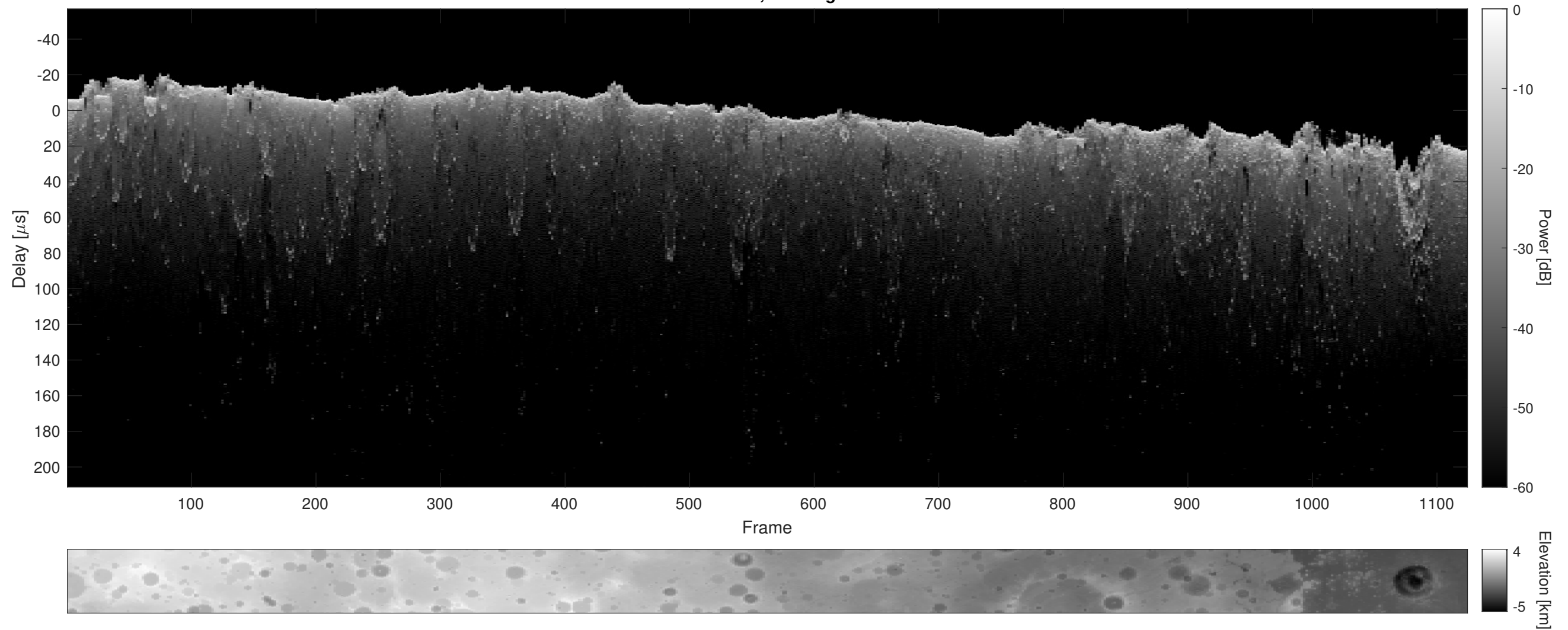
Orbit 22861, Cluttergram
