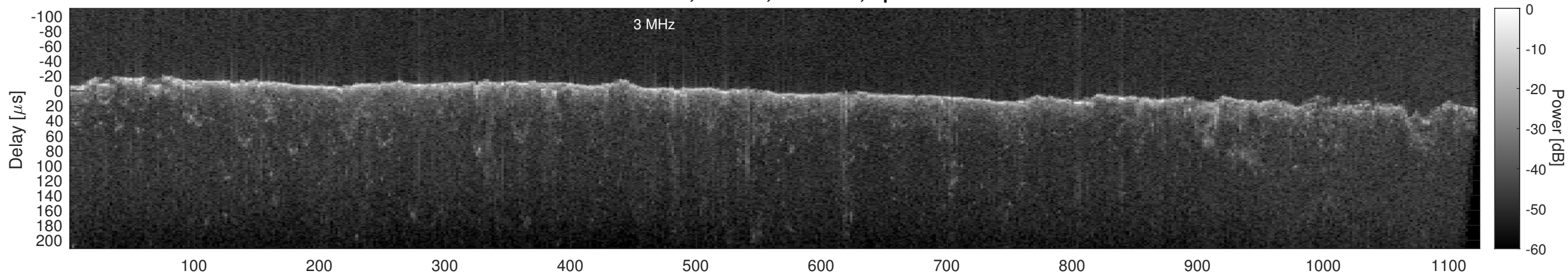
Orbit 22861, Cluttergram
