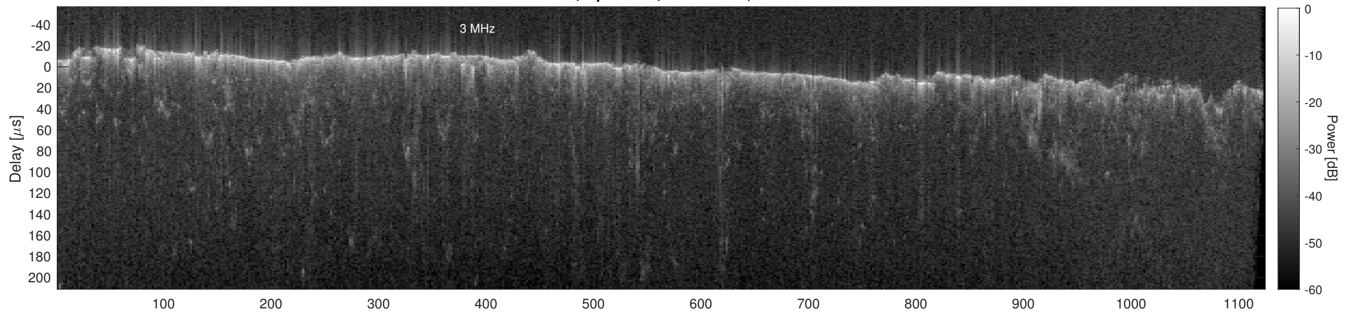
Orbit 22861, Cluttergram
