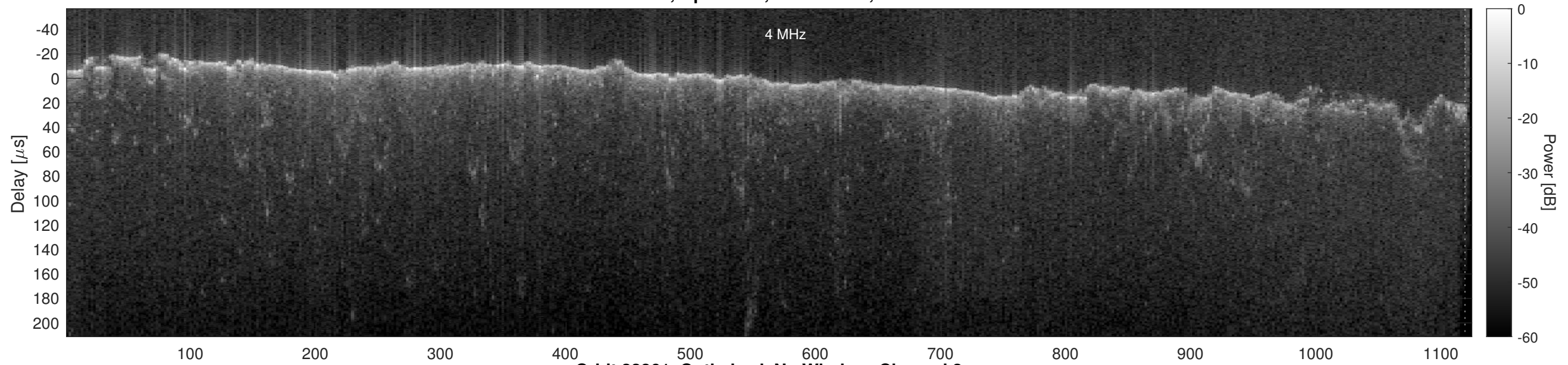
Orbit 22861, Optimized, No Window, Channel 2
