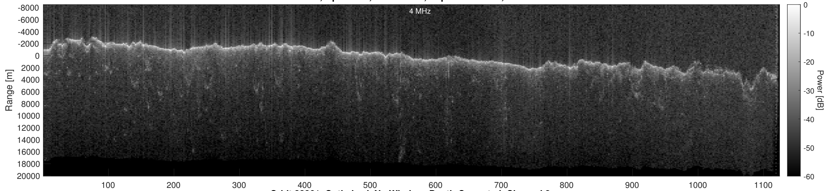
Orbit 22861, Optimized, No Window, Depth-Corrected, Channel 2
