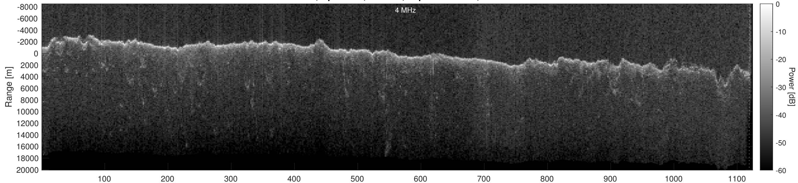
Orbit 22861, Optimized, Window, Depth-Corrected, Channel 2
