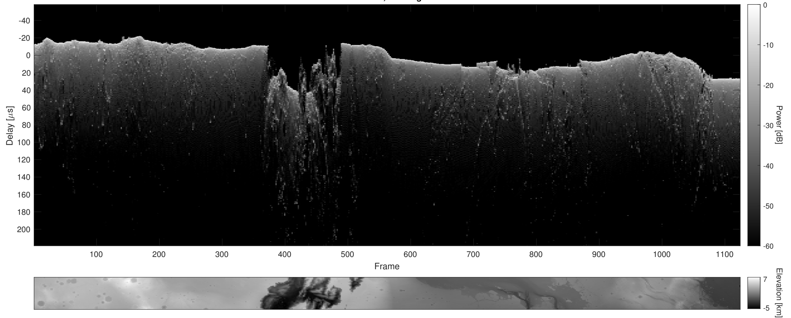
Orbit 22862, Cluttergram
