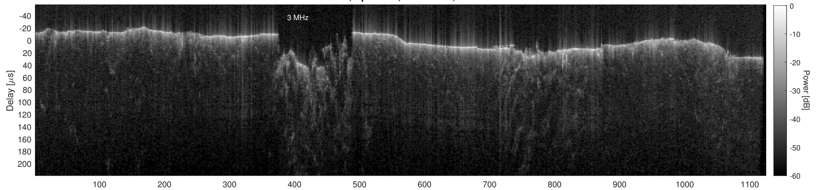
Orbit 22862, Cluttergram
