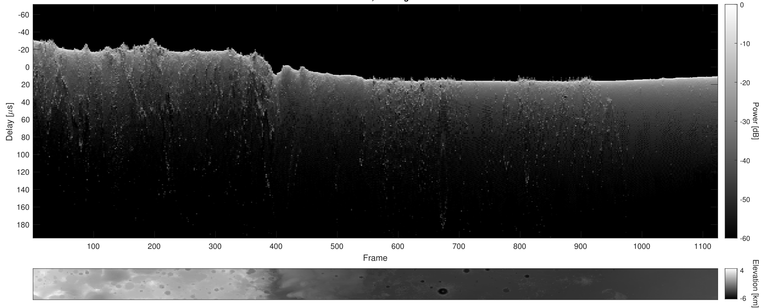
Orbit 22863, Cluttergram
