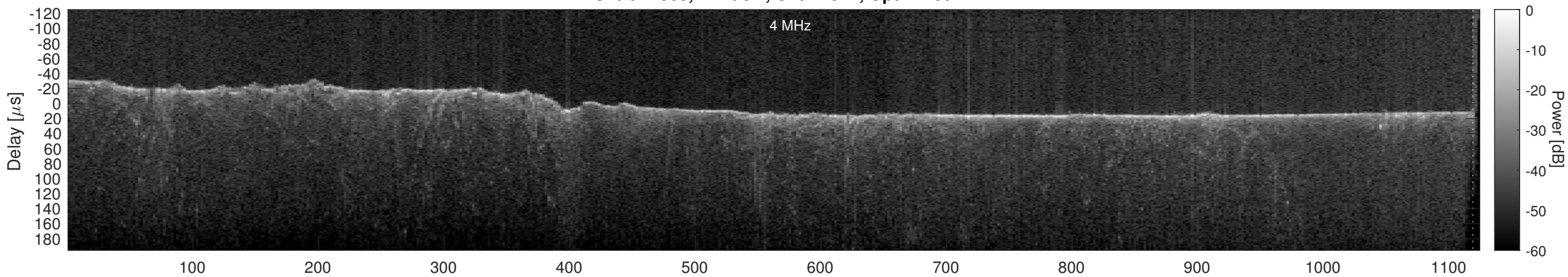
Orbit 22863, Cluttergram
