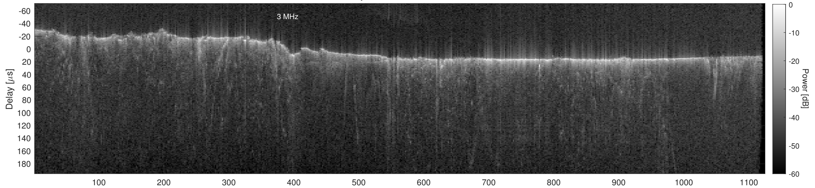
Orbit 22863, Cluttergram
