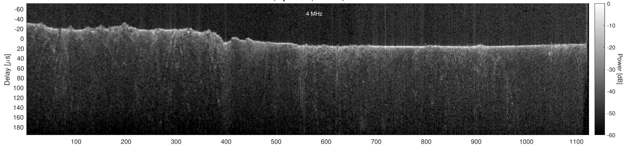
Orbit 22863, Optimized, Window, Channel 2
