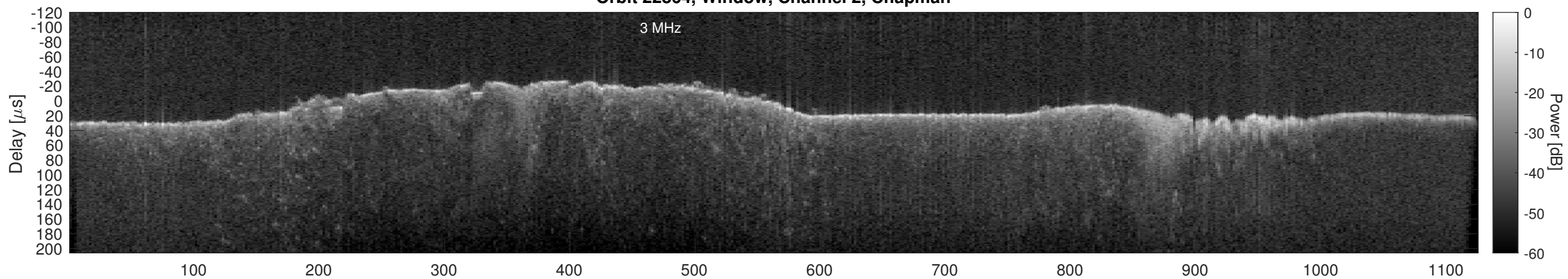
Orbit 22864, Window, Channel 2, Optimized
