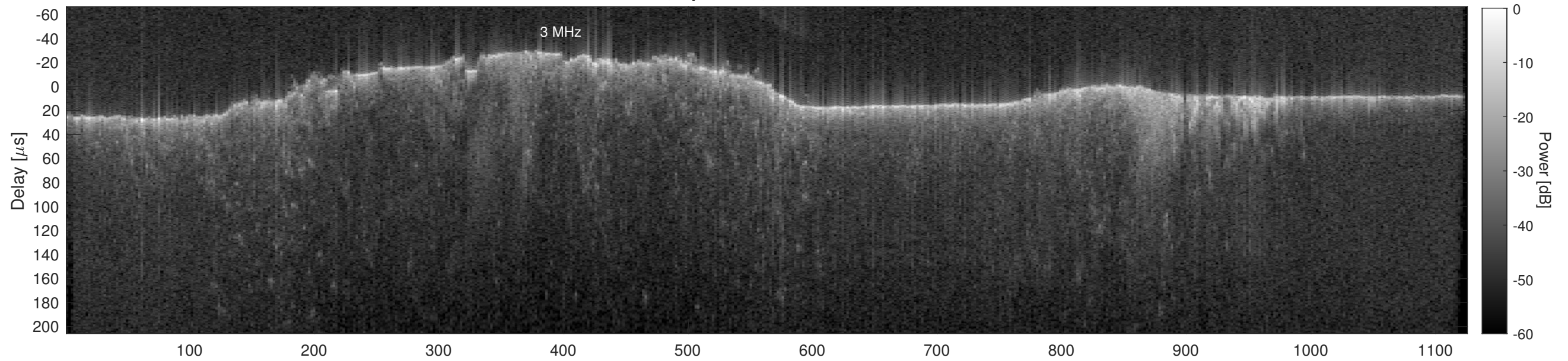
Orbit 22864, Cluttergram
