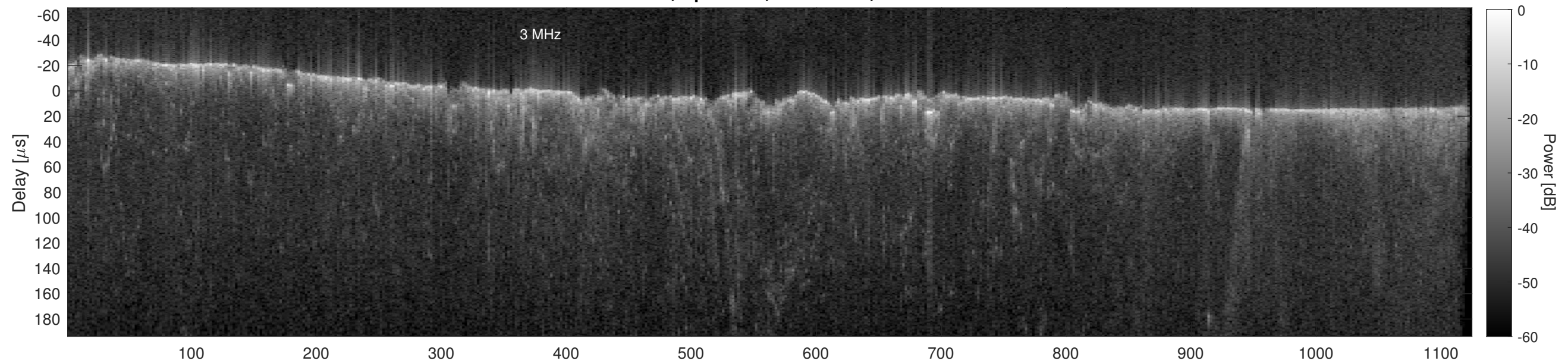
Orbit 22865, Cluttergram
