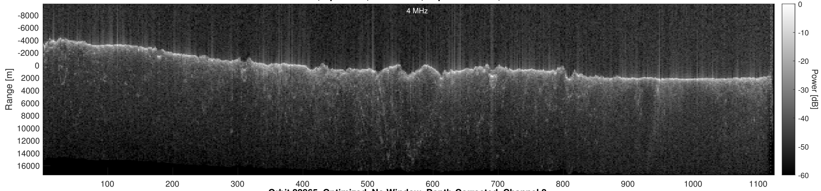
Orbit 22865, Optimized, No Window, Depth-Corrected, Channel 2
