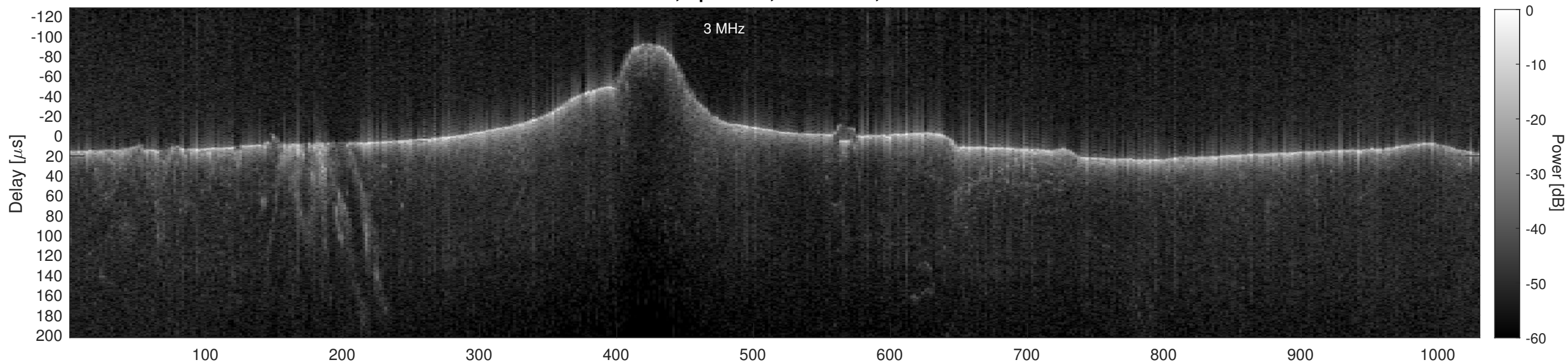
Orbit 22866, Cluttergram
