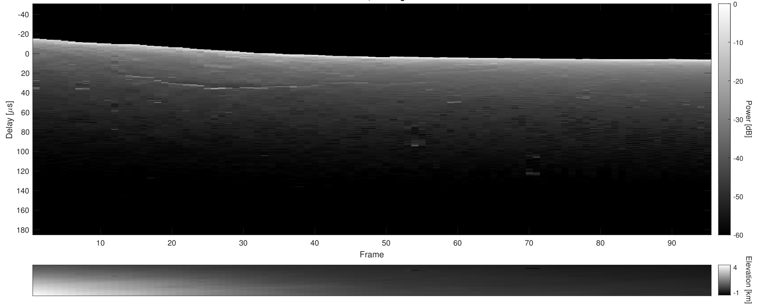
Orbit 22867, Cluttergram
