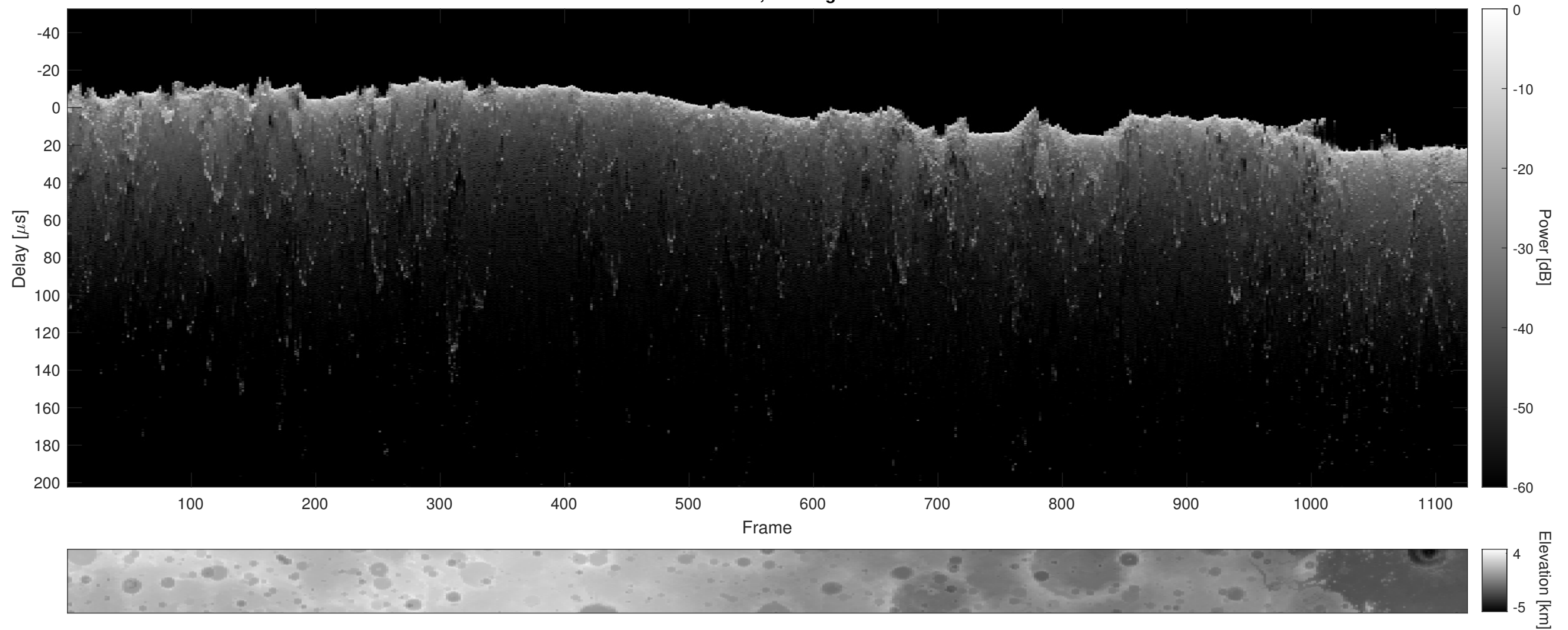
Orbit 22868, Cluttergram
