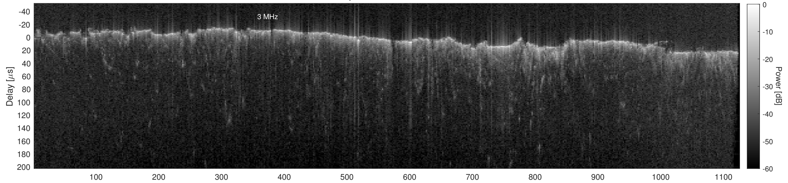
Orbit 22868, Cluttergram
