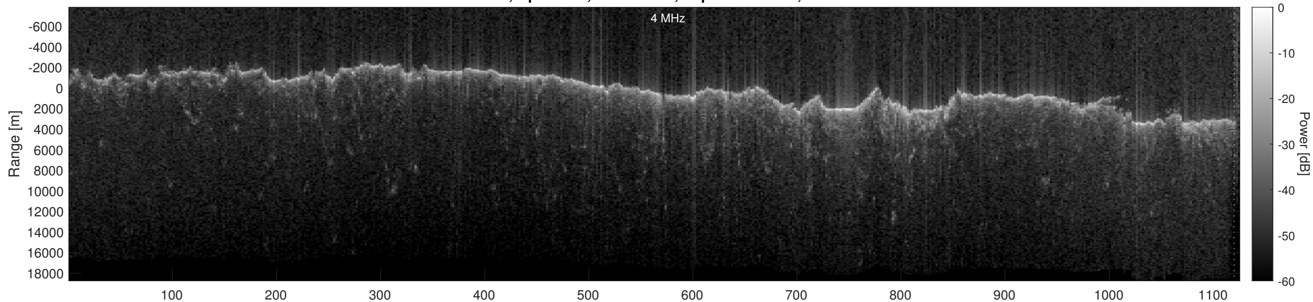
Orbit 22868, Optimized, No Window, Depth-Corrected, Channel 2
