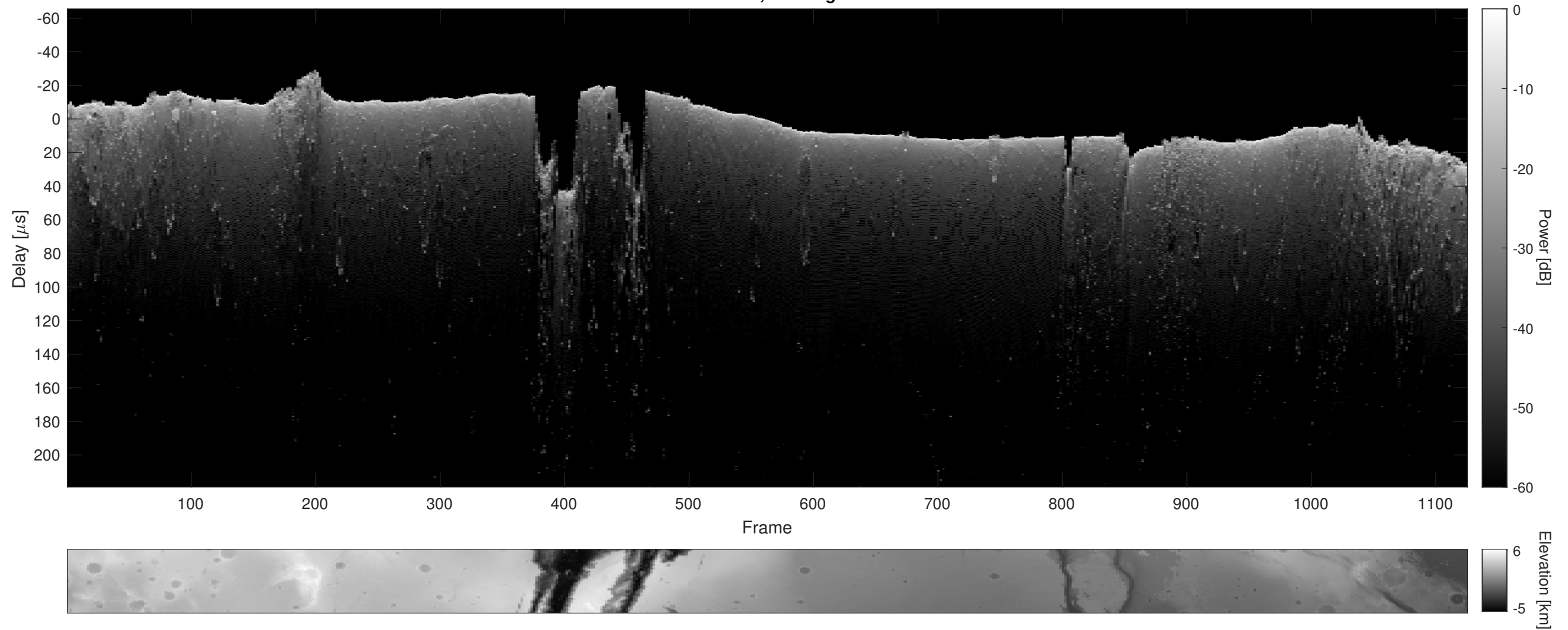
Orbit 22869, Cluttergram
