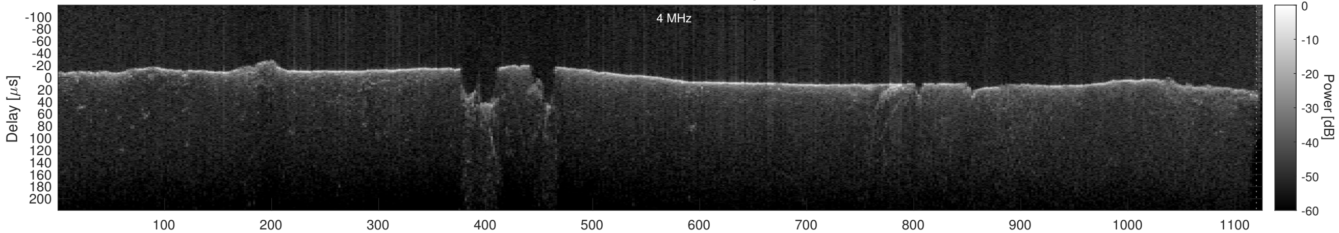
Orbit 22869, Cluttergram
