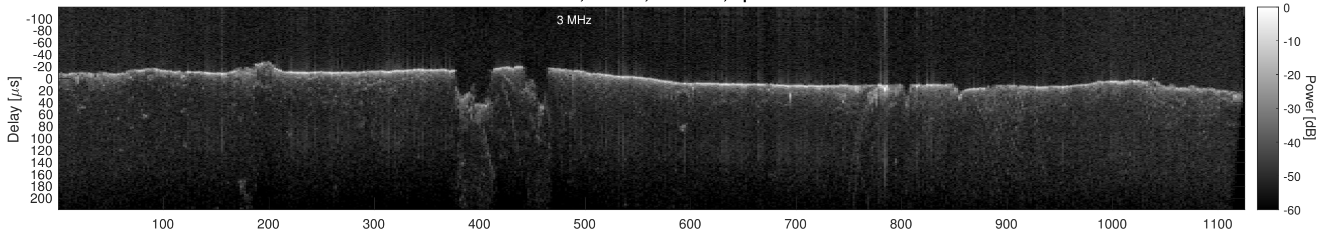
Orbit 22869, Cluttergram
