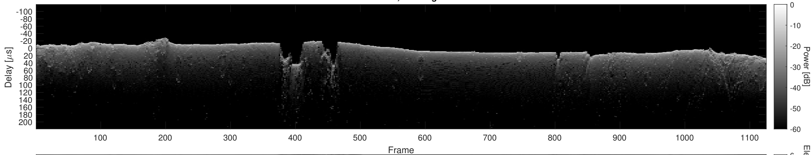
Orbit 22869, Cluttergram
